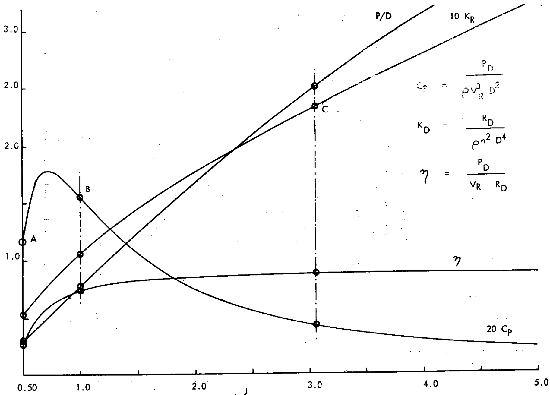
FIG 5 WINDMILL PERFORMANCE CURVES
